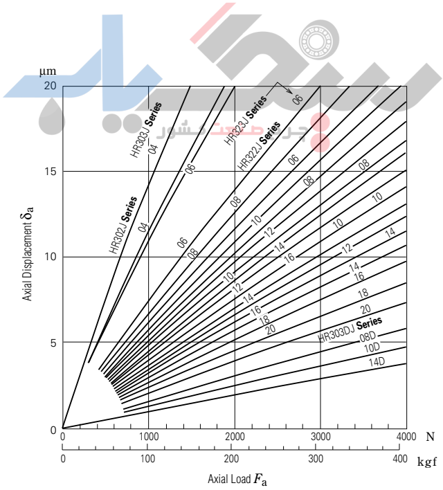
Fig. 15.4 Axial Load and Axial Displacement of Tapered Roller Bearings
