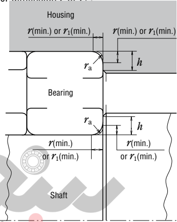
Fig. 11.1 Chamfer Dimensions, Fillet Radius of Shaft and Housing, and Shoulder Height
