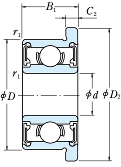
Non-Contact Sealed Type VV
