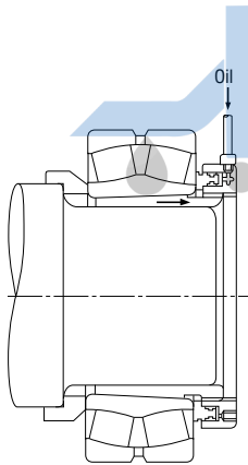
Fig. 14.20 Removal Using Hydraulic Nut
