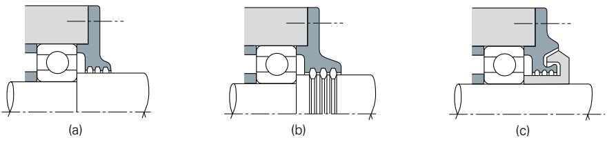
Fig. 11.5 Examples of Oil Grooves
