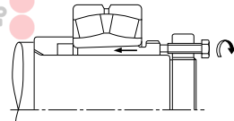
Fig. 14.5 Mounting with Withdrawal Sleeve
