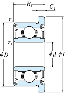
Shielded Type ZZ · ZZ1
