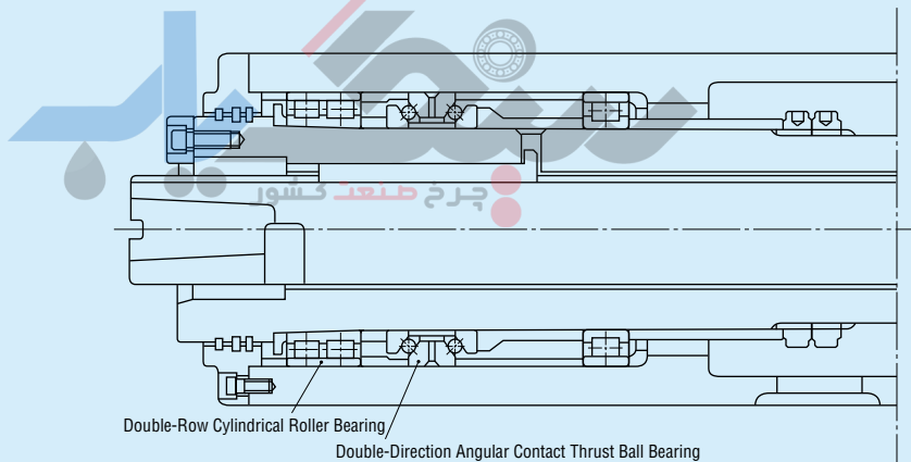
Example of Application of Double-Direction Angular Contact Thrust Ball Bearing (Main Spindle of Machine Tool)
