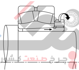
Fig. 14.16 Removal of Withdrawal Sleeve Using Withdrawal Nut (1)
