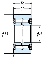
Full Complement
