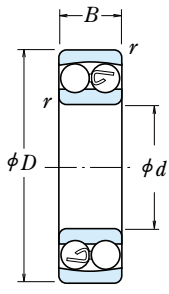
Cylindrical Bore
