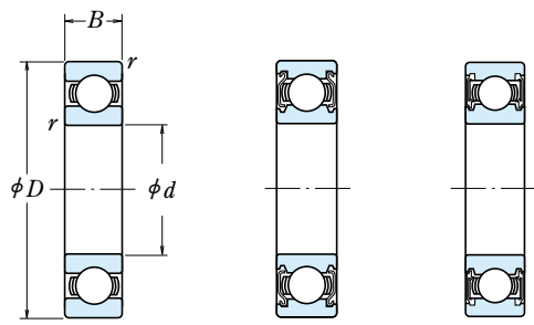
Shielded Type ZS
