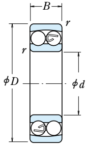
Cylindrical Bore
