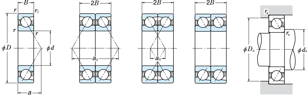
Single Back-to-Back DB Face-to-Face DF Tandem DT
