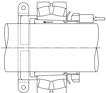
Fig. 14.18 Removal of Adapter with Stop and Axial Pressure
