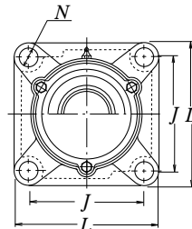
Cast dust cover type
