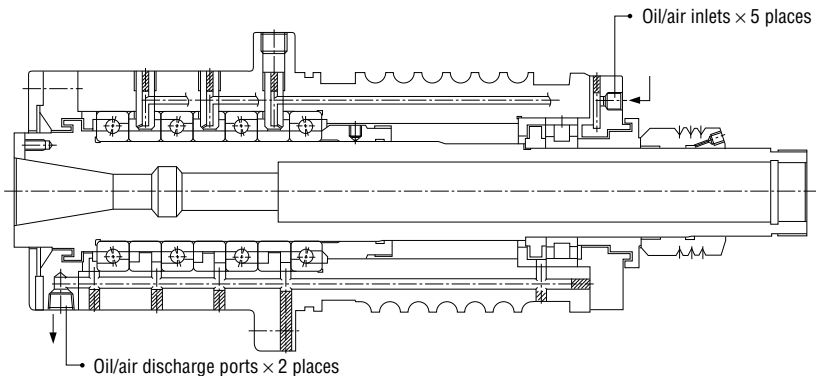
Fig. 12.10 Oil/Air Lubrication
