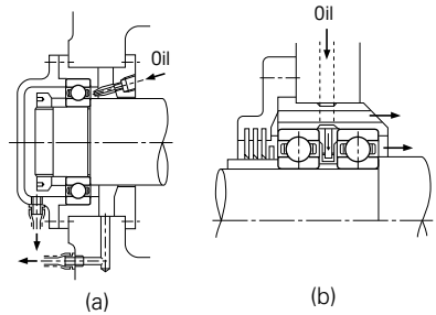
Fig. 12.8 Jet Lubrication
