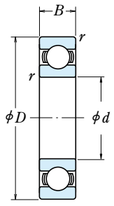
Open Type
