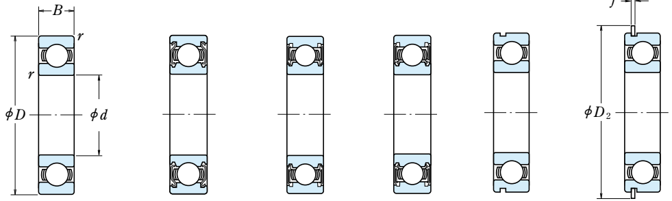
Open Type Shielded Type ZZ Non-Contact Sealed Type VV Contact Sealed Type DD · DDU With Snap Ring Groove N With Snap Ring NR
