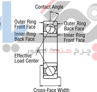
Single-Row Angular Contact Ball Bearing
