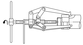
Fig. 14.14 Removal of Inner Ring Using Withdrawal Tool (2)
