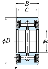
Full Complement, Sealed with Thrust Washer
