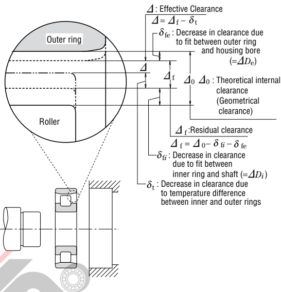
Fig. 9.2 Changes in Radial Internal Clearance of Bearings
