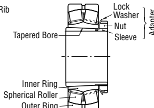
Spherical Roller Bearing
