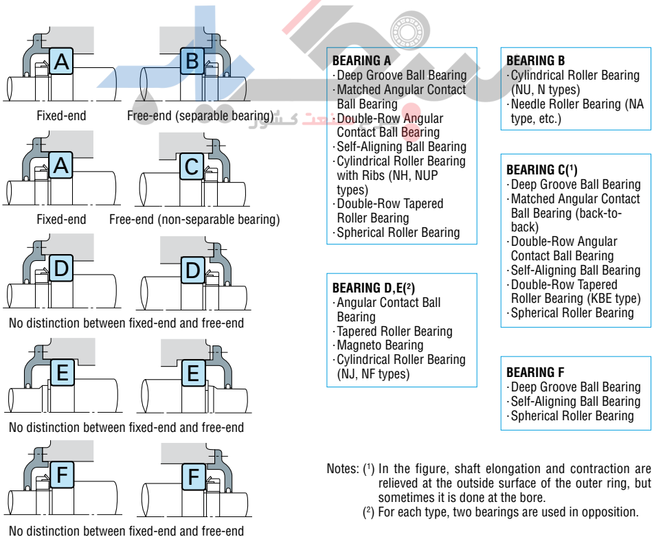
Fig. 4.1 Bearing Mounting Arrangements and Bearing Types
